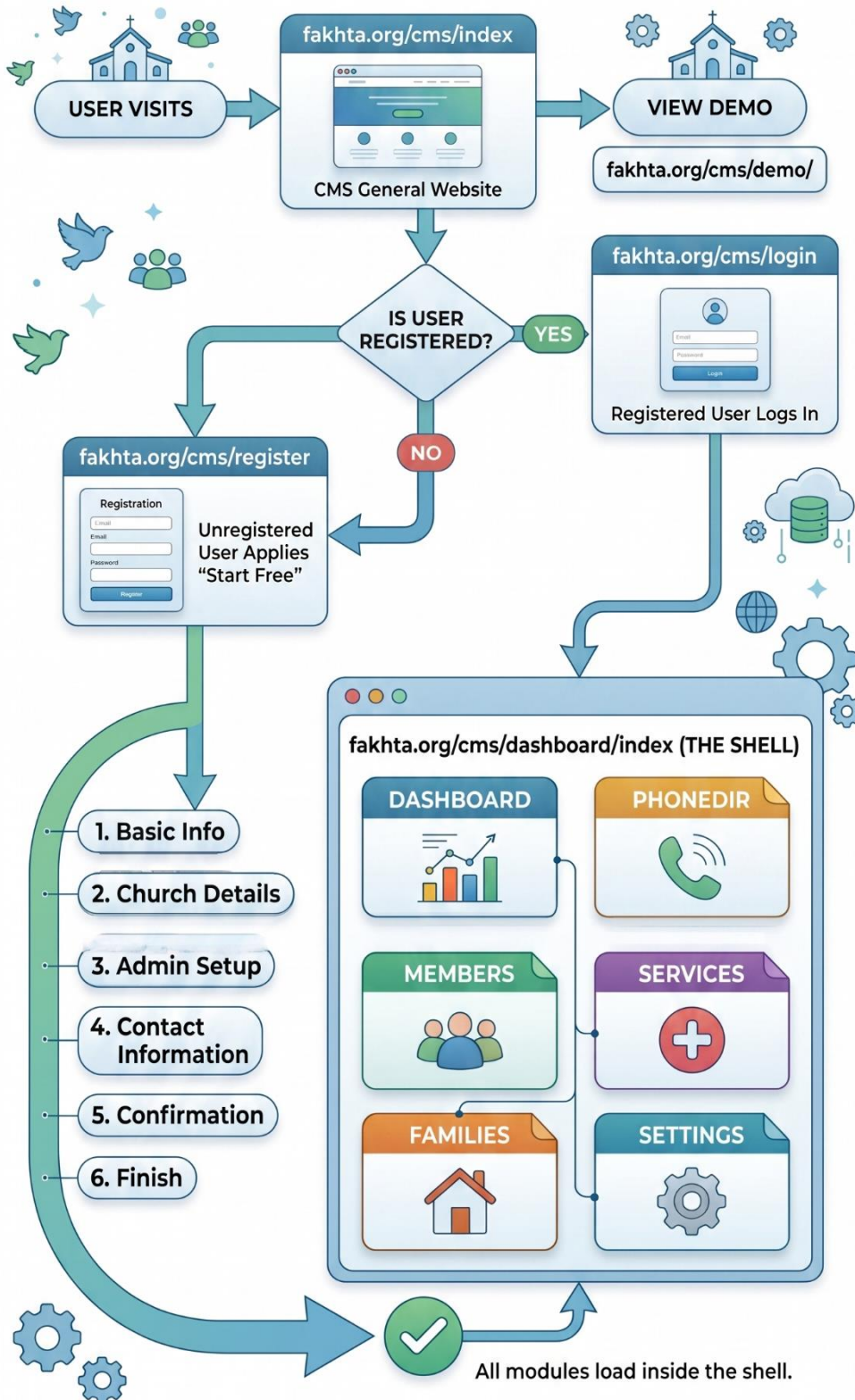
Fakhta Church Management System Flowchart
